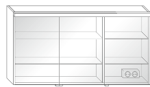
SPLA/SPLB L/R H 640 x T 180 x B 1100, 1200, 1300, 1400 mm
